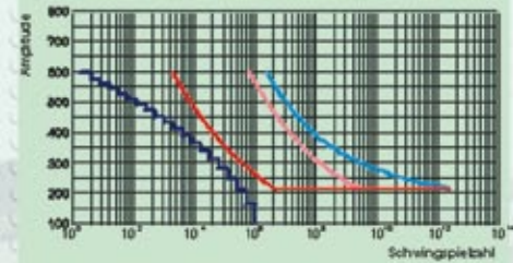
Wöhlerkurve
